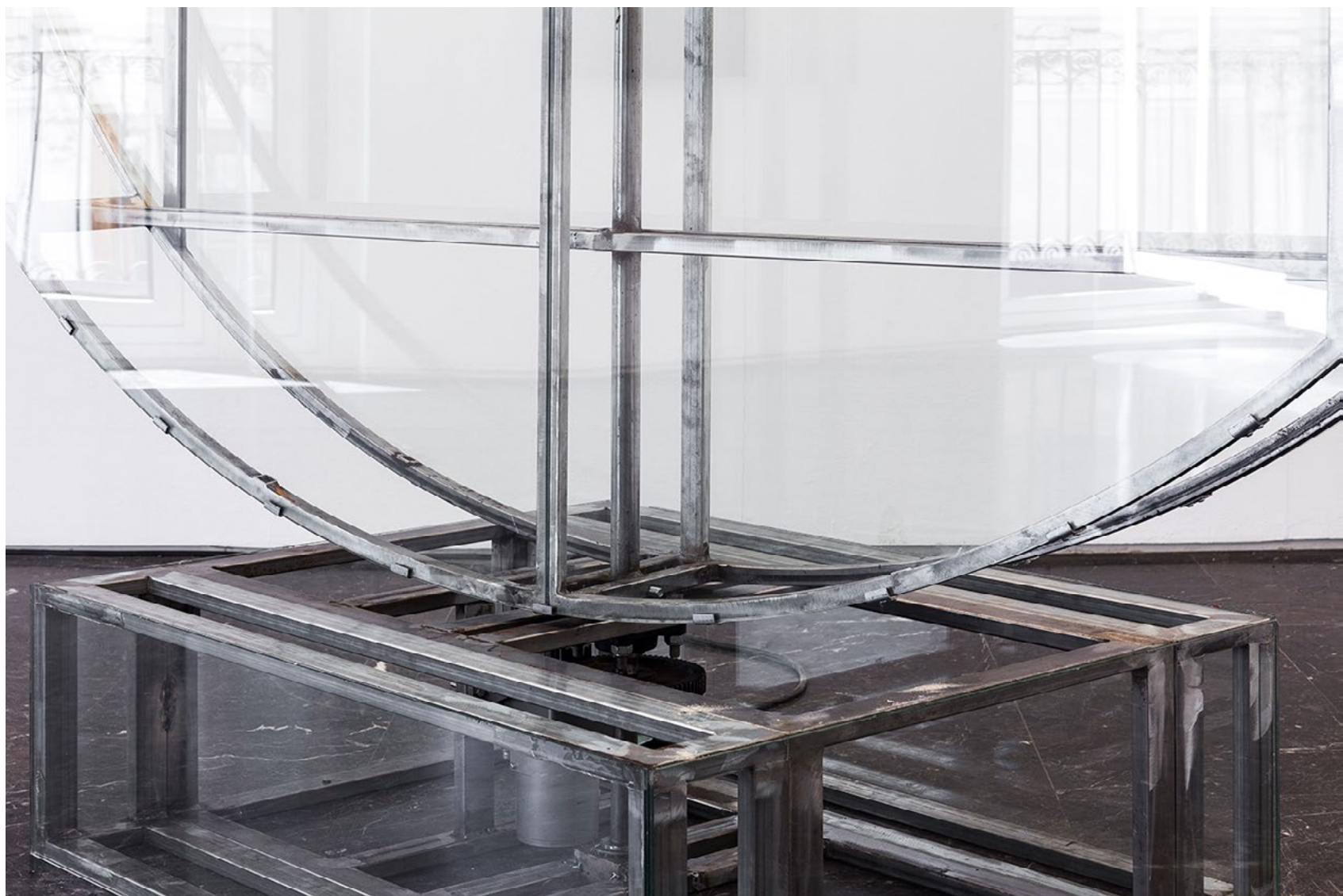
Disco cristal , 2018. Metallic profile 20 x 20 x 2 mm. 2 circumferences of 2.5 mt joined with structure of metallic profile composed of 6 horizontal and vertical bars of 40 x 20 cm. Round central axis 30 x 1.5 cm. Laminated glass cover 3 + 3 worked with hammer blows and other objects. Compound of 4 pieces. Base: Profile 20 x 40 x 1000 x 800 mm. Conical bearing diameter 40 mm. Flat bearing diameter 25 mm. Toothed gear 80 teeth. Toothed gear 20 teeth. Calibrated 25 mm. Motor Oriental Motors 30 MegaNewton
